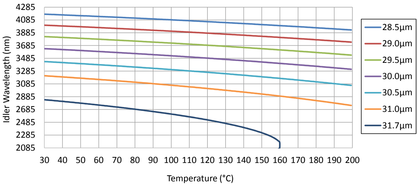
OPO Tuning Curve 1064nm Pump
