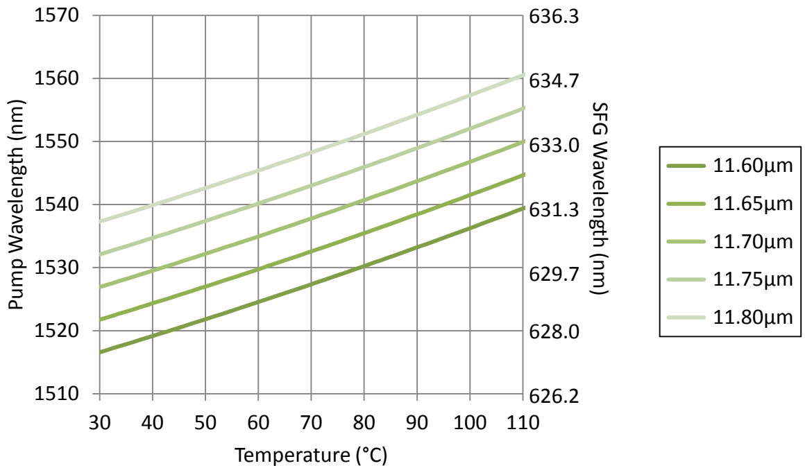
SFG Tuning Curve for 1070nm Pump
